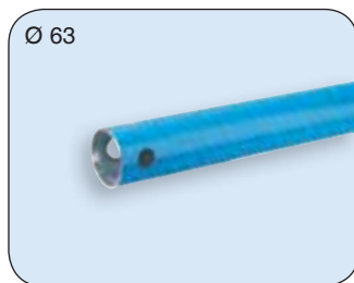
Pipe pre-drilled at each end with two 22mm diameter holes, deburred and chamfered
